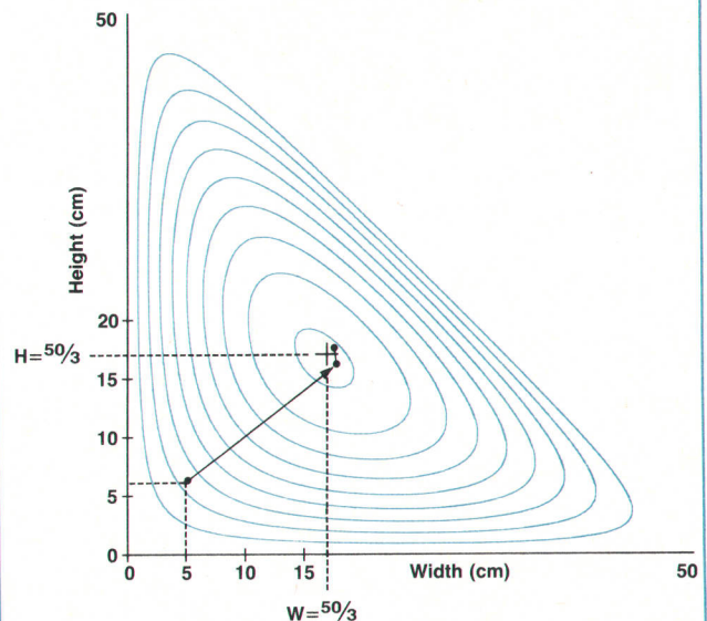
Fig. 2. Plot of constant volume contours for Equation (1). Maximum volume occurs when H = W = 16.6667 cm.
